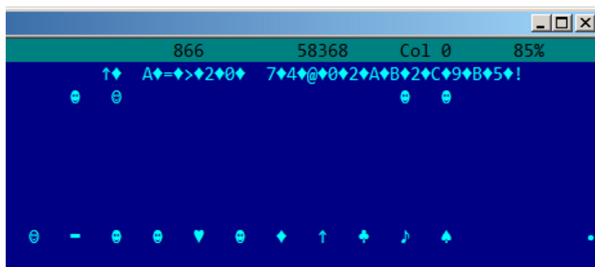
Рис. 5.5: Hiew: UTF-16LE
