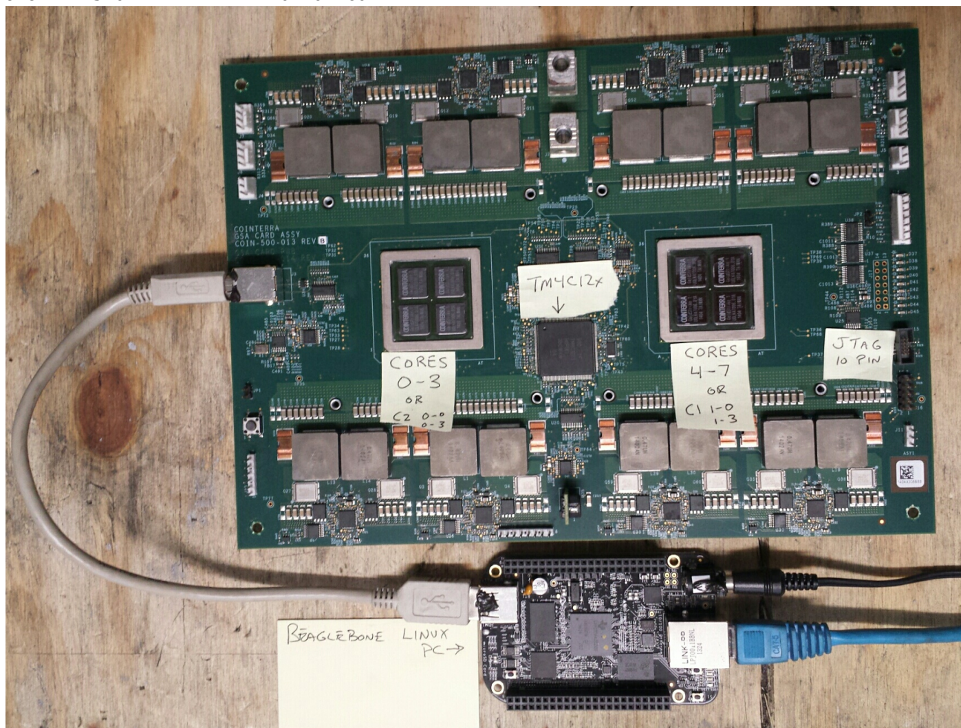
Рис. 8.14: Board
