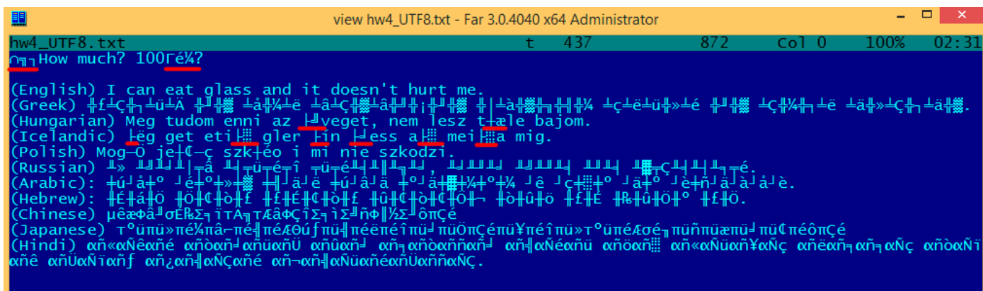
Рис. 5.2: FAR: UTF-8
