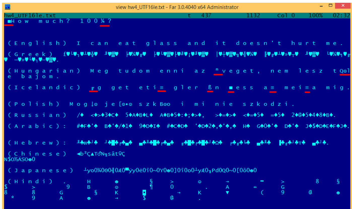
Рис. 5.6: FAR: UTF-16LE
